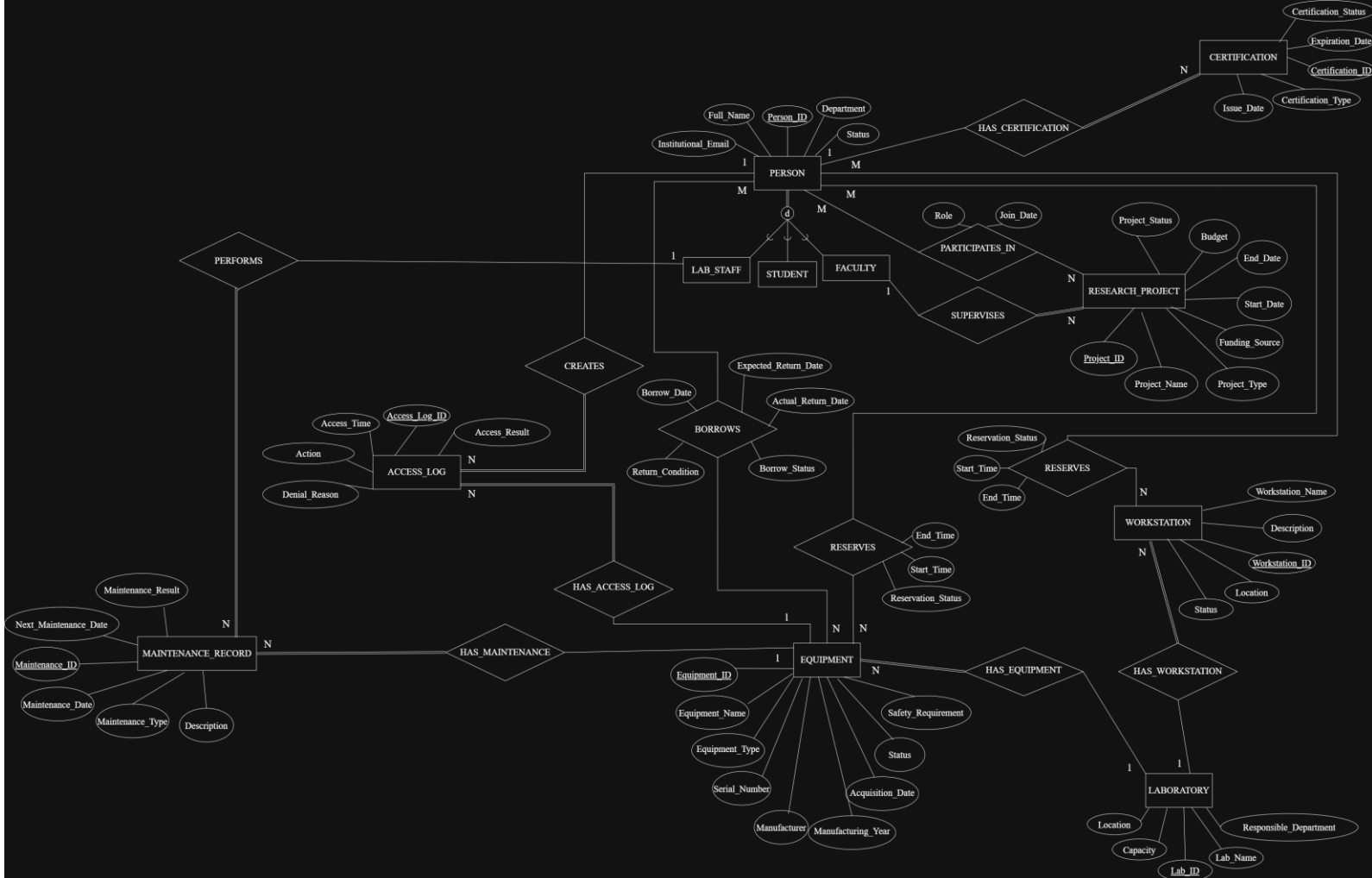
Hình 1. Conceptual EER Diagram – University Physics Laboratory Asset Tracker
